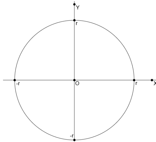
Figure 4: Metrica d'(x, y)
